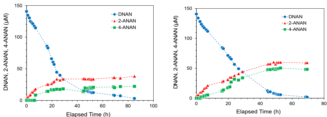
Fig. 3.2.3. Concentrations of DNAN, 2-ANAN, and 4-ANAN ( \mu\text{M} ) vs. elapsed time (h) during two replicate biodegradation experiments with bacterial enrichment culture MBR.
