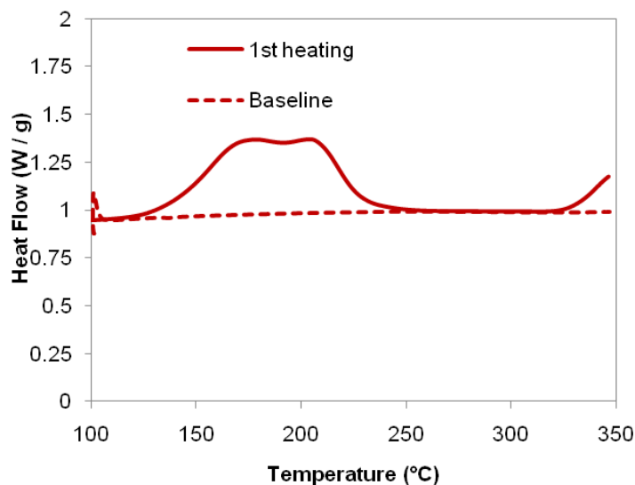
Figure 12. DSC scan of uncured 11 .
