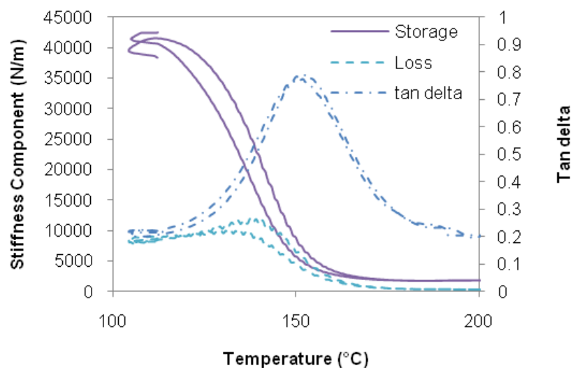
Figure 14. Oscillatory TMA scan of cured (10) (dry)
