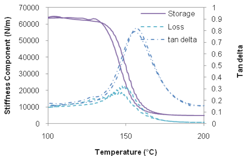
Figure 15. Oscillatory TMA scan of (10) after exposure to 85 °C water for 96 hrs.
