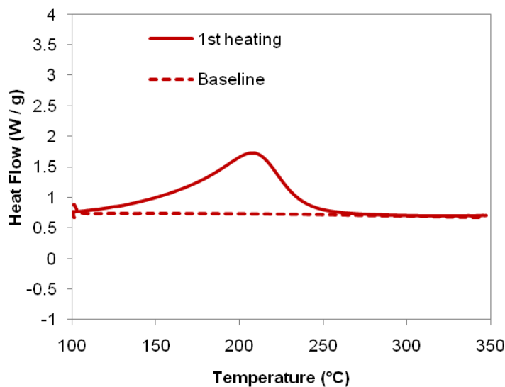
Figure 11. DSC scan of uncured 10 .
