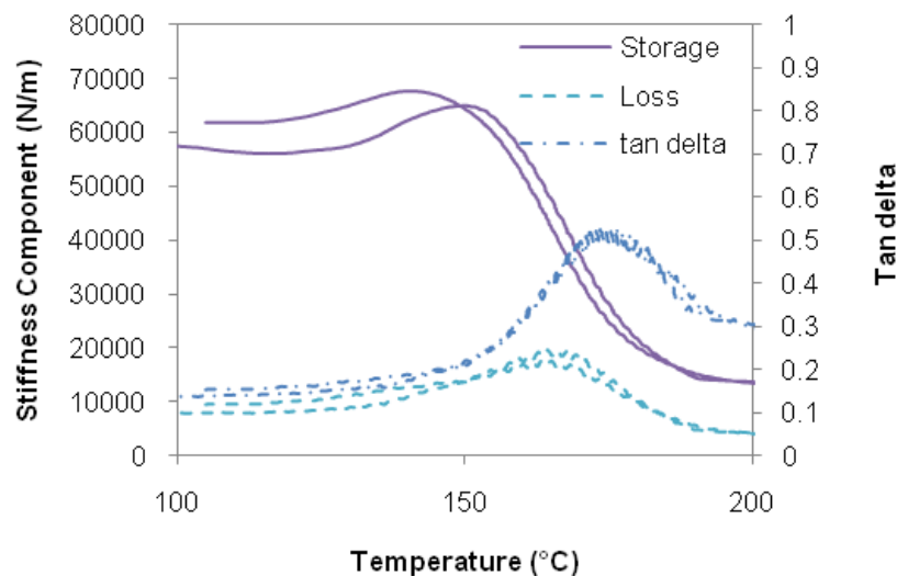
Figure 17. Oscillatory TMA of cured ( 11 ) after exposure to 85 °C water for 96 hrs.
