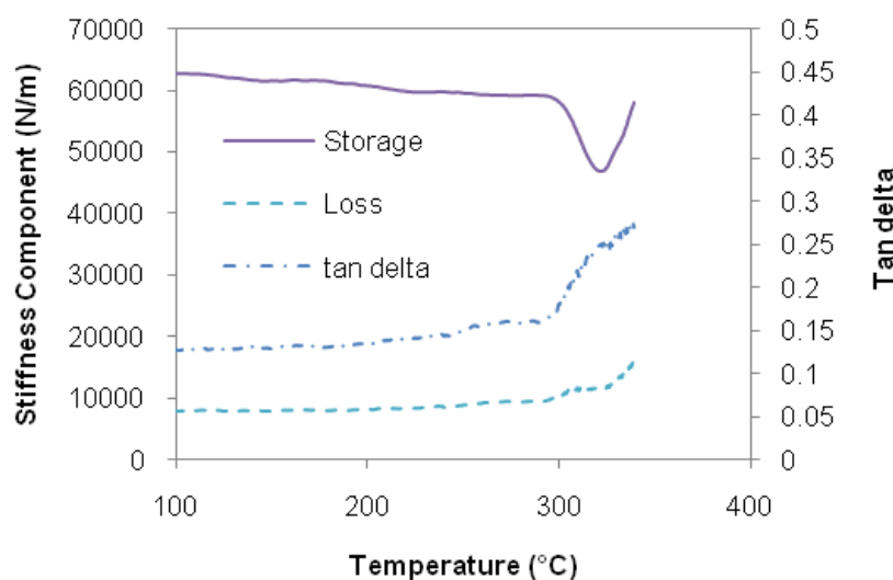
Figure 16. Oscillatory TMA of cured ( 11 ) (dry).
