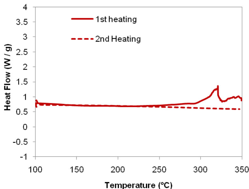
Figure 13. Residual cure of (11) as measured by DSC.
