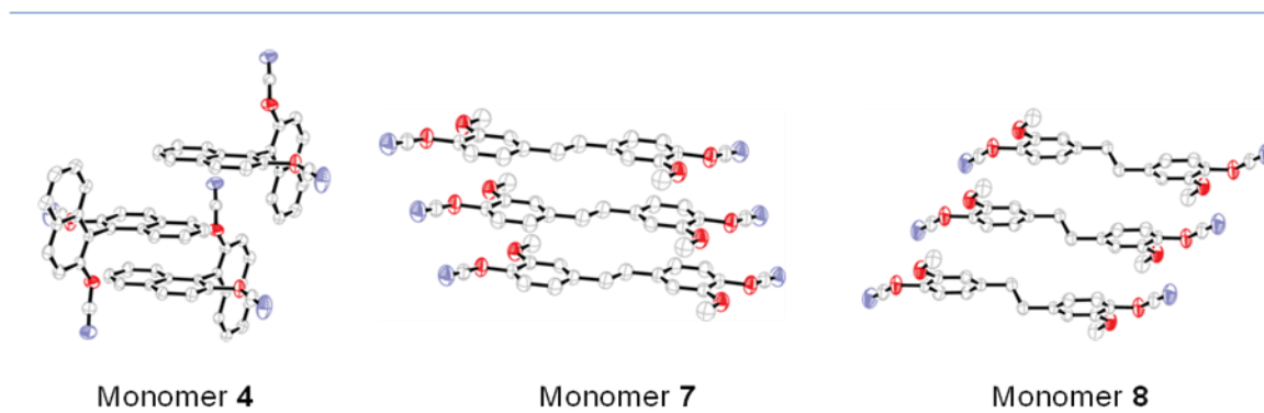
Figure 6. ORTEP drawings of 2,2'-bis(2-cyanato)-1,1'-naphthyl) ( 4 ), 1,2- E -bis(4-cyanato-3-methoxyphenyl)ethene ( 7 ), and 1,2-bis(4-cyanato-3-methoxyphenyl)ethane ( 8 ) taken from the single-crystal x-ray diffraction molecular-structure determinations.
